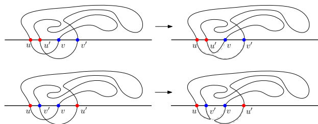
Figure 4: Replacing edges uv and u'v' by edges uv' and u'v .
