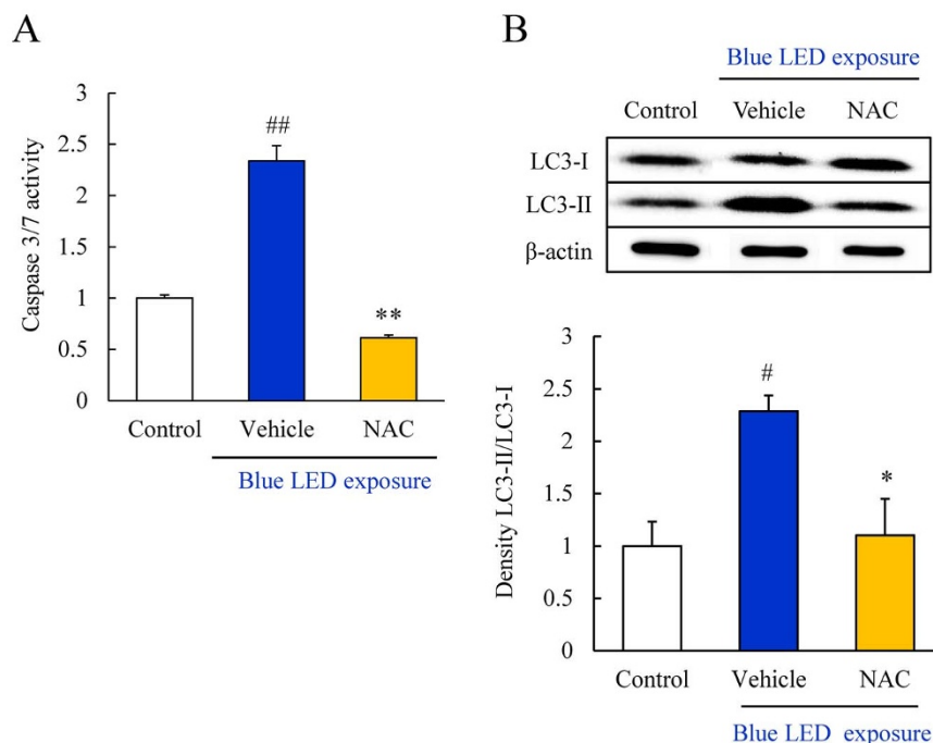
Figure 7 | NAC suppressed blue LED light-induced caspase-3/7 activation and autophagy activation. (A) Measurement of caspase-3/7 activity by Caspase-Glo® 3/7 Assay kit. Activation of caspase-3/7 was observed after blue LED light exposure. NAC treatment significantly inhibited the activation. Data are expressed as mean ± SEM (n = 3 or 4). ** indicates p < 0.01 vs. vehicle; ## indicates p < 0.01 vs. control (one-way ANOVA followed by Tukey's test). (B) Western blots of LC3-II/LC3-I indicated an increase in the expression level after blue LED light exposure. NAC treatment significantly reduced the expression. Data are expressed as mean ± SEM (n = 6). * indicates p < 0.05 vs. vehicle; # indicates p < 0.01 vs. control (one-way ANOVA followed by Tukey's test). The cropped blots are used in this Figure and the full-length blots are presented in Supplementary Figure S9.
