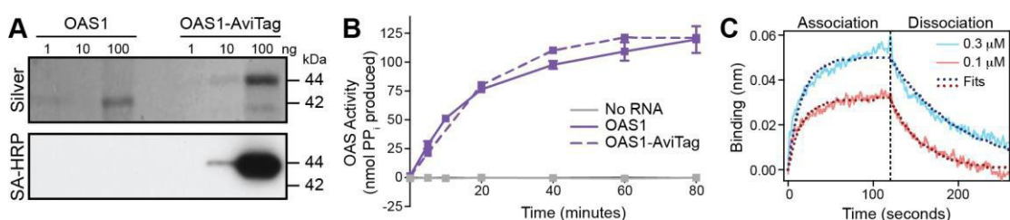
Fig. 4. OAS1-AviTag is active and can be biotinylated for BLI assays. A , Serially diluted wild-type OAS1 and OAS1-AviTag were analyzed by SDS-PAGE and visualized using silver stain ( top ) or blotted with streptavidin-horseradish peroxidase ( bottom ). B , OAS1 activation by the “wild-type”
