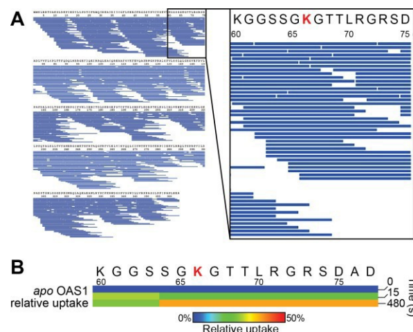
Fig. 5. Preliminary HDX-MS data. A , OAS1 mapping experiment demonstrating the potential for acquiring high quality HDX-MS data (100% coverage, 33-fold redundancy).
