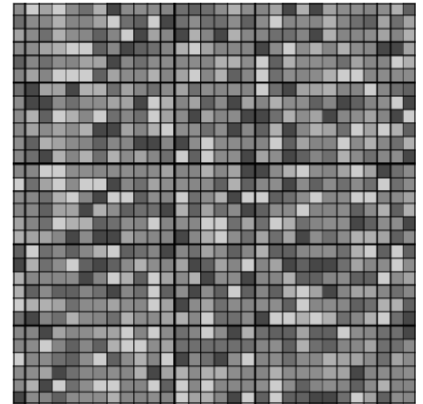
Digits of \pi represented by grey tones
