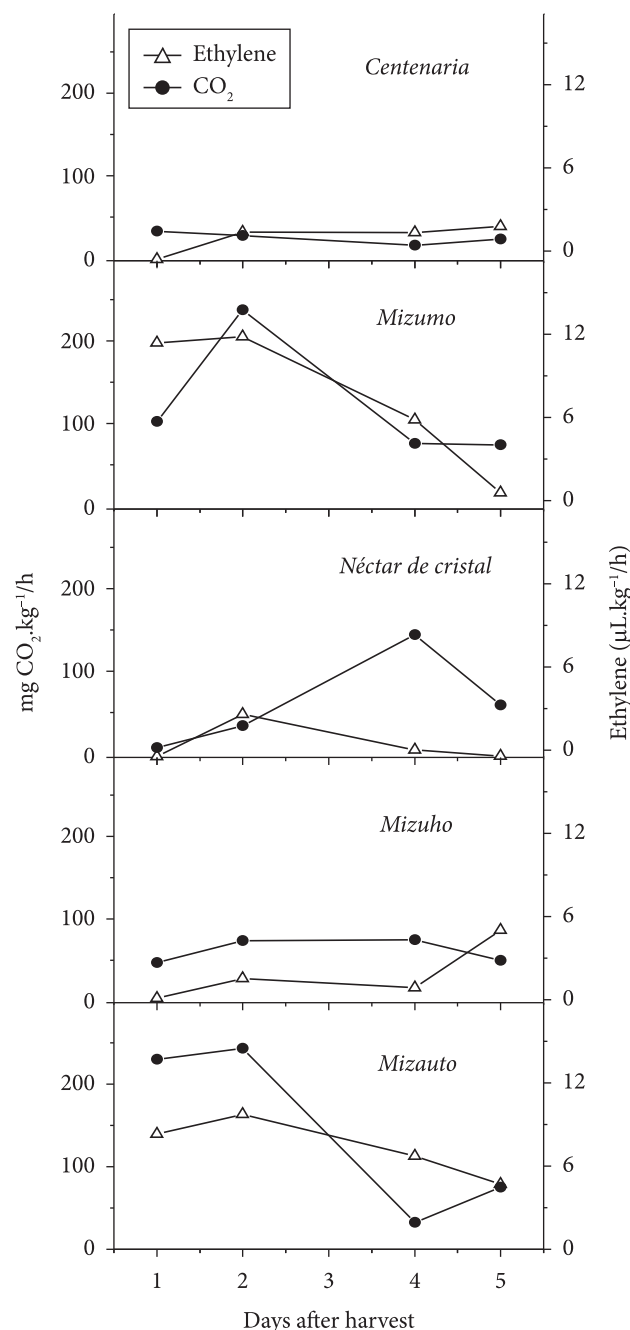
Figure 1. Respiration (—●—) and ethylene production (---△---) profiles after fruit harvest for five loquat cultivars. The data are means \pm standard deviation of three replicates.
