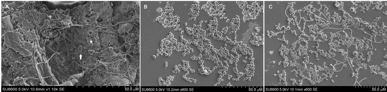
Fig. 4: (A) scanning electron micrograph of a 48 h old, Candida albicans biofilm in RPMI 1640 medium. Note the architecture of 72 h old mature biofilm with profuse extracellular matrix (M), hyphal elements (white solid arrow) blastospores (★), some bearing bud-scars (+) (Scale indicates 50.0 μM); (B) scanning electron micrograph of a 48 h old, C. tropicalis biofilms in RPMI 1640 medium. Note the architecture of 72 h old mature biofilm devoid of extracellular matrix and relatively sparse growth compared to Fig. 4A above (Scale indicates 50.0 μM); (C) scanning electron micrograph of a 48 h old, 1:1 mixed species biofilm of C. albicans and C. tropicalis in RPMI 1640 medium devoid of extracellular matrix but clearly showing hyphal elements of C. albicans intermixed with C. tropicalis blastospores devoid of hyphae (Scale indicates 50.0 μM).
