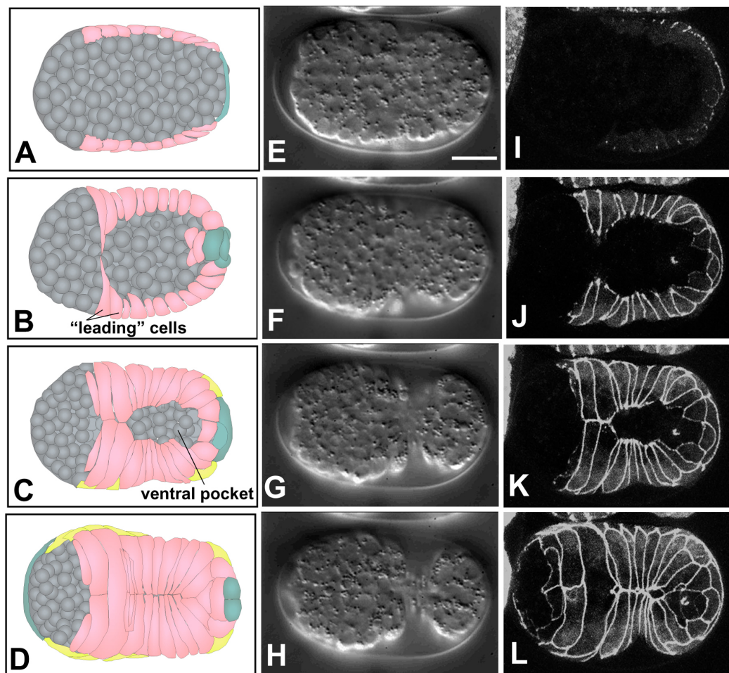
Figure 4. Epidermal enclosure. Schematics (left column, A-D), Nomarski images (middle column, E-H, ventral view; see also Movie 5 ) and DLG-1::GFP images (right column, I-L, ventral view; see also Movie 6 ) of ventral enclosure. Different embryos, at corresponding developmental stages, are shown in middle and right columns. Scale bar = 5 \mu m. Ventral cells are shown in pink in the left-hand column; seam epidermal cells in yellow, and dorsal cells, which wrap around the tail, in teal. Neuroblasts and other internal cells are depicted in gray. The first two pairs of ventral cells to reach the ventral midline are termed “leading cells” ( Williams-Masson et al., 1997 ), which extend long protrusions towards the midline (B). After the leading cells make contact at the ventral midline, cells posterior to these cells, termed “pocket cells” ( Williams-Masson et al., 1997 ), reach the midline (C). Finally, the anterior epidermal cells enclose the head (D).
