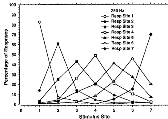
Figure 7. Localization of sites on a 7-tactor linear array on the forearm; 25 mm separation, 100 Hz (upper graph) and 250 Hz (lower).
