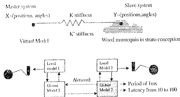
Figure 2. Distant control of the robot in position
