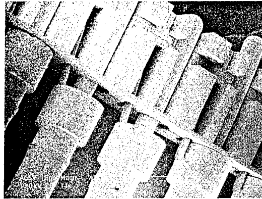
Figure 3. REM picture that shows the design and position of the slider, which serves to pull the clamping springs, thereby releasing the taxels
