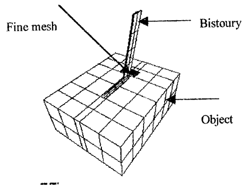
Figure 2. Modelling of the cutting problem
