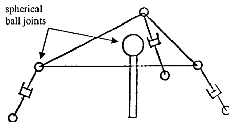
Figure 3 – the PARAMAT structure
