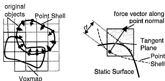
Figure 1: Voxmap-PointShell-Model TM
