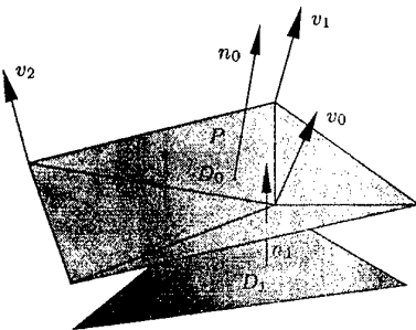
Figure 3: Overlapping triangles.
