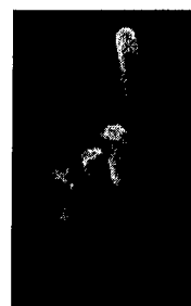
Figure 4. Index-Finger-Stroke
