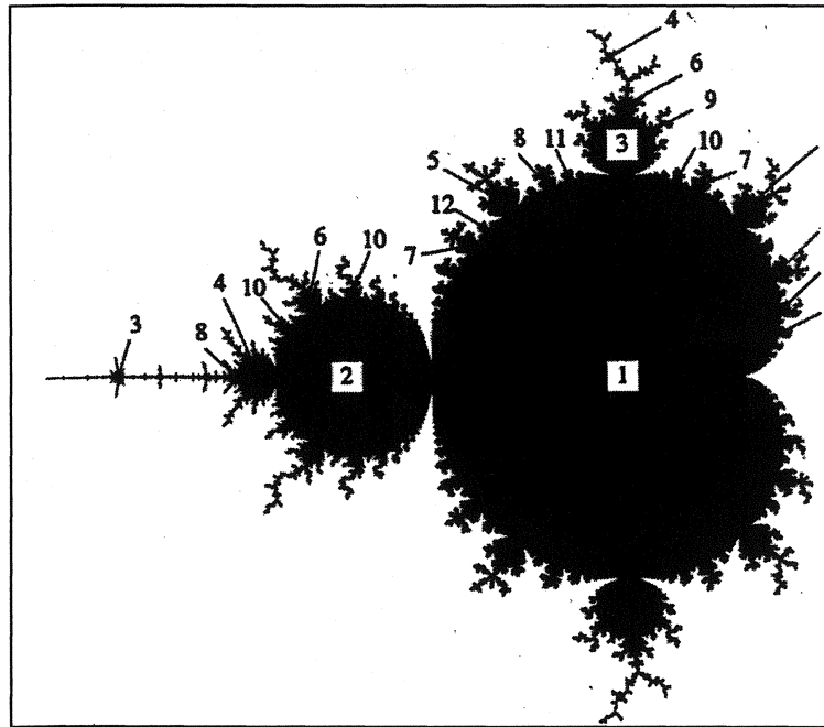
Figure 3: The Mandelbrot set.
