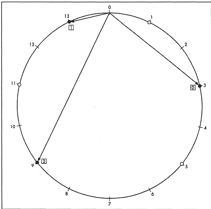
Figure 4: The points k shown with closed circles within the following 14-gon represent the edge-lengths from point 0 to point k of the star 14-gon \{14/k\} . These are elements of the trajectories of the logistic equation corresponding to that 14-gon. The open circles represent the mirror image trajectory. The numbers in square boxes are the order of the points in the trajectory.
