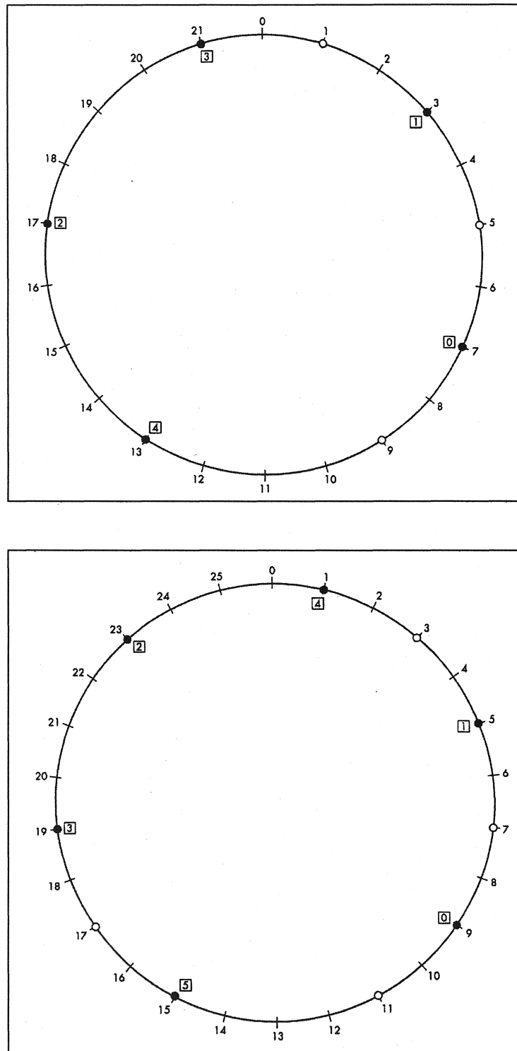
Figure 5: Trajectories of the logistic equation corresponding to the edges of (a) a star 22-gon; (b) a star 26-gon (see figure caption of Figure 4).
