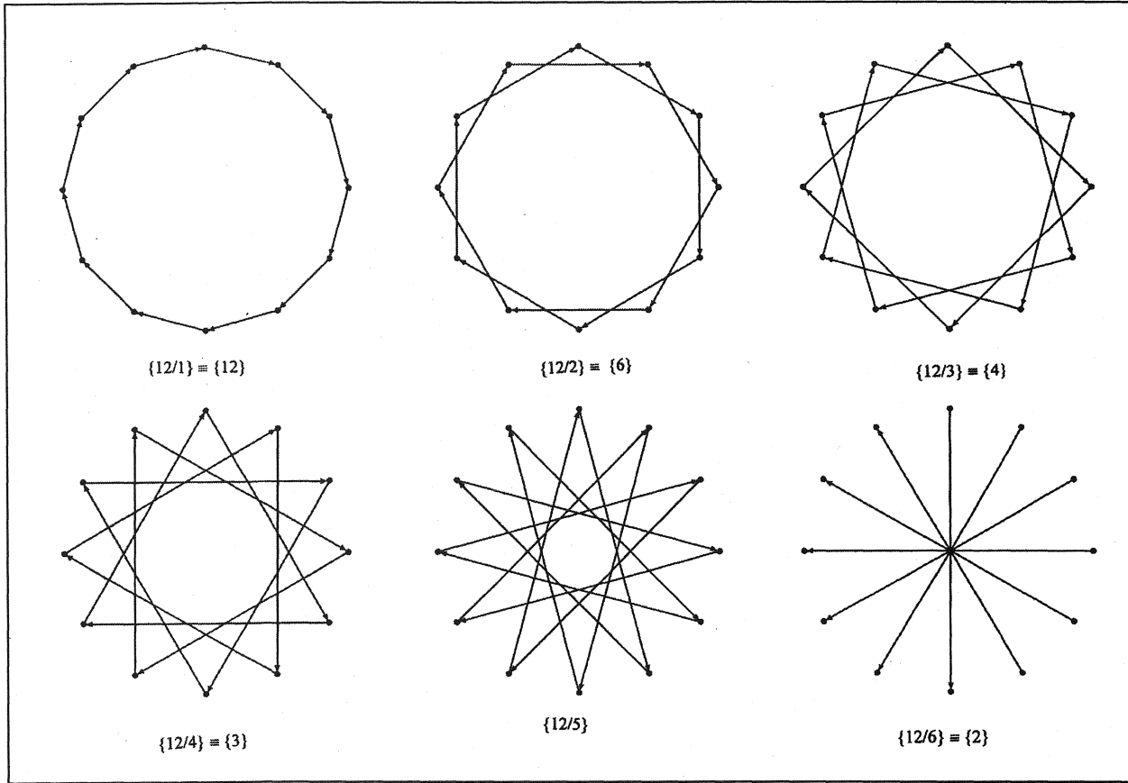
Figure 2: The family of star 12-gons. Only \{12\} and \{12/5\} are star 12-gons. The star polygons \{12/3\} \equiv \{4\} is a 4-gon, \{12/4\} \equiv \{3\} is a 3-gon, and \{12/6\} \equiv \{2\} is a digon.
