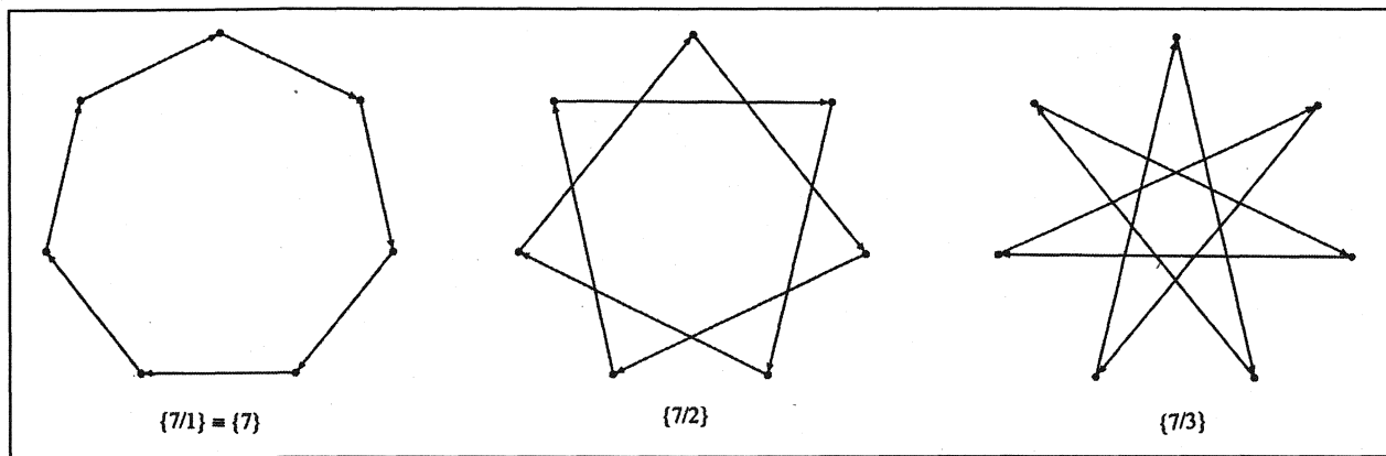
Figure 1: The three positively oriented 7-gons.
