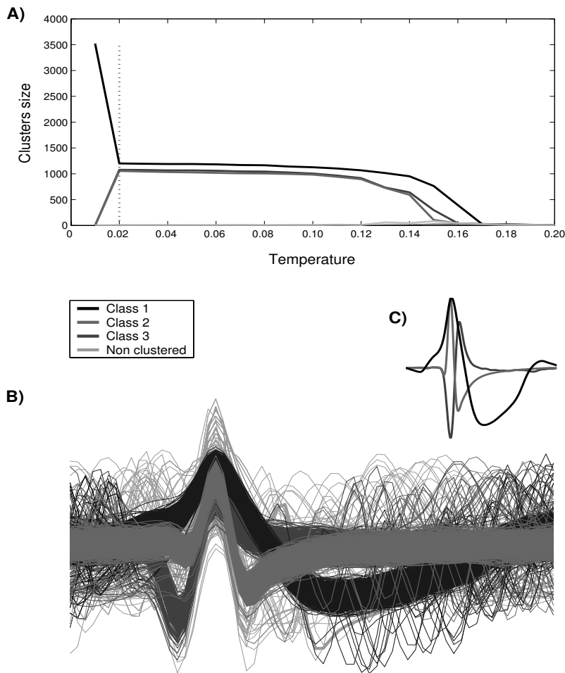
Figure 9: (A) Cluster size vs. temperature. Based on the stability criterion of the clusters, a temperature of 0.02 was automatically chosen for separating the three spike classes. (B) All spikes with gray levels according to the outcome of the clustering algorithm. Note the presence of overlapping spikes. (C) Original spike shapes.
