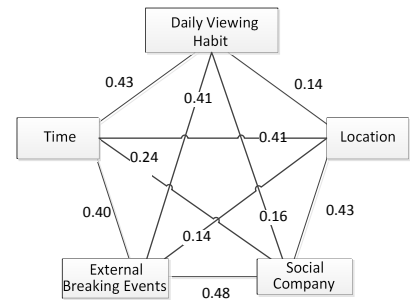
Figure 4: Pearson Correlation Coefficient of Different Pair of Factors
