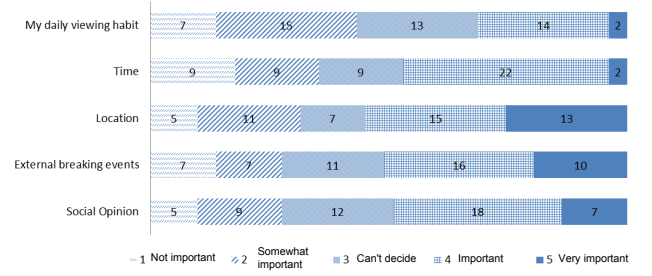
Figure 3: Users' Scoring Distribution on Contextual Factors' Importance
