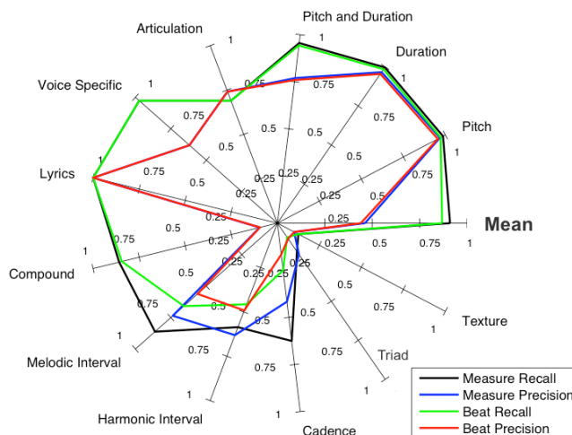
Figure 2. Results of the Stravinsqi-Jun2014 algorithm on the MediaEval 2014 C@merata task. Overall results are indicated by the mean label, and followed by results for twelve question categories.
