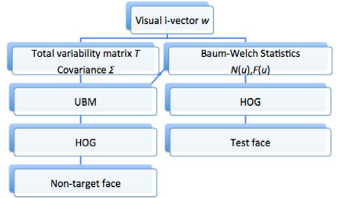
Figure 1: Overview of visual i-vector extraction
