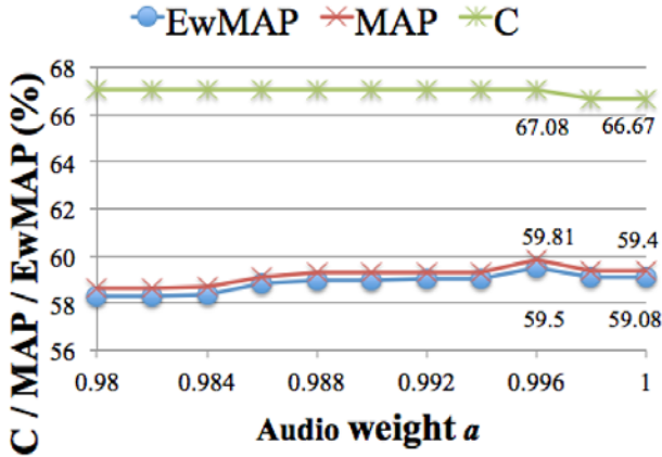
Figure3: EwMAP, MAP, C by audio weight a in development set.
