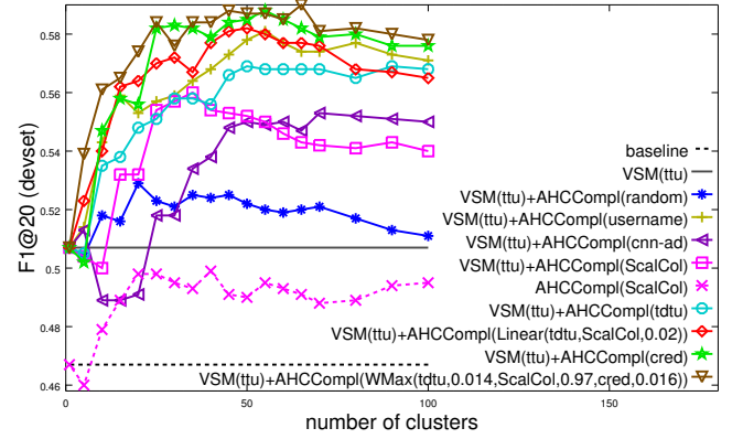
Figure 1: Some of the results on devset varying the number of clusters (300 documents per query)
