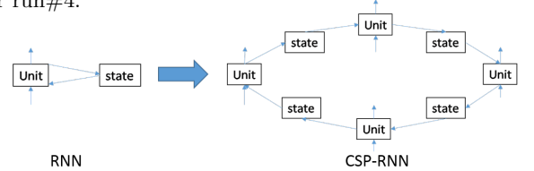
Figure 2: Proposed CSP-RNN structure.
