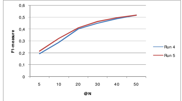
Figure 3. F1-measure comparison between Run 4 and Run 5
