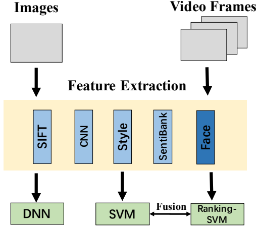
Figure 1: An overview of the key components in our proposed methods. We use DNN and SVM for both subtask, while Ranking-SVM is only used in video subtask. The face feature is computed according to the movement of face in the video shot, which is also only used in video subtask.
