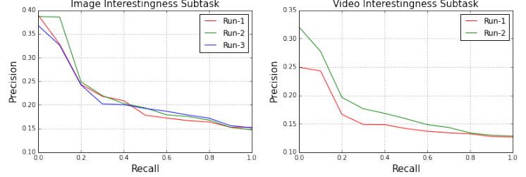
Figure 3: Tabulated Results in (a) and Precision-Recall curve of two subtasks
