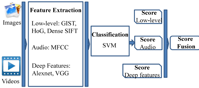
Figure 1: Our framework for extracting and encoding local features.
