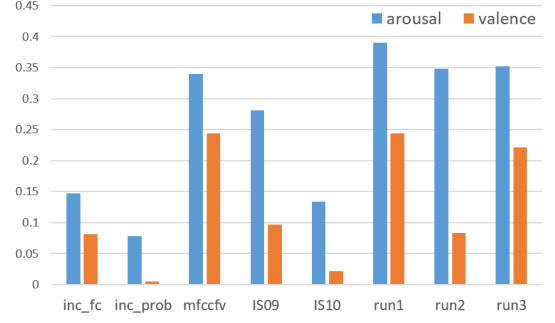
Figure 3: PCC Performance of Different Features for Continuous Prediction on Local Testing Set
