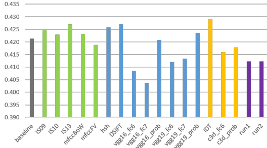
Figure 2: MSE Performance of Different Features for Global Valence Prediction on Local Testing Set
