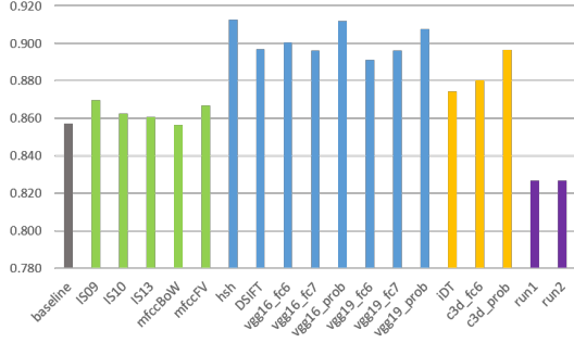
Figure 1: MSE Performance of Different Features for Global Arousal Prediction on Local Testing Set
