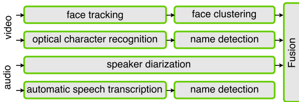
Figure 2: Multimodal baseline pipeline.
