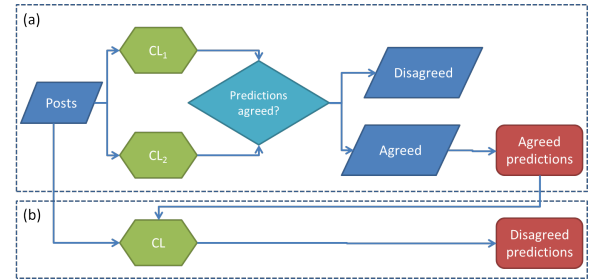
Figure 1: Overview of agreement-based retraining.
