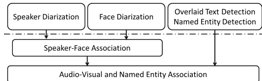
Figure 1: Architecture of our system
