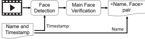
Figure 3. <Name, Face> Pair Identification Process
