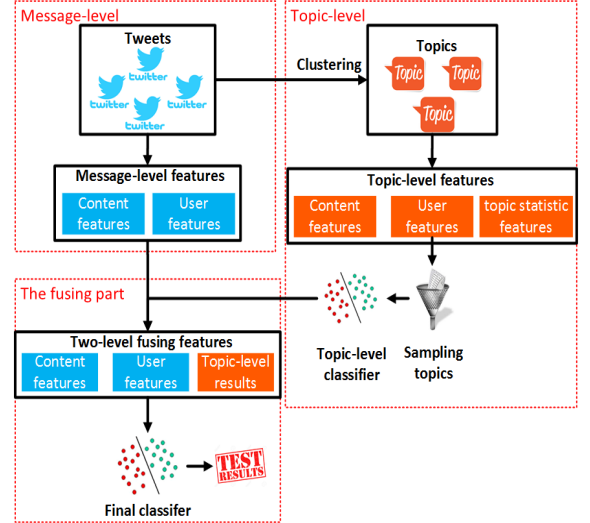
Figure 1: The framework of the text analysis approach
