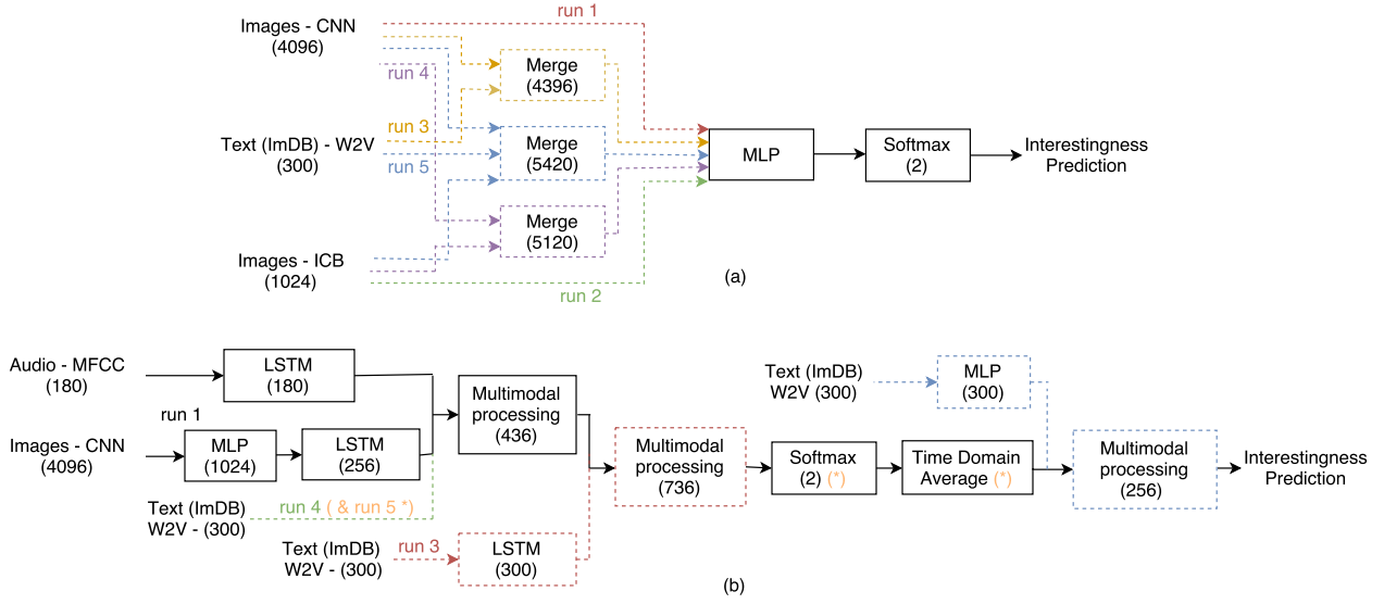
Figure 1: Workflows for all run submissions: (a) image subtask. (b) video subtask. *: block swapping.
