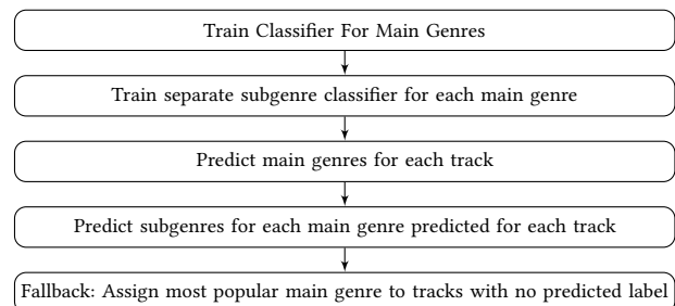
Figure 1: Classification workflow for subtask 1.
