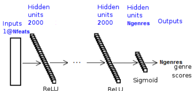
FIGURE 1: DNN architecture
