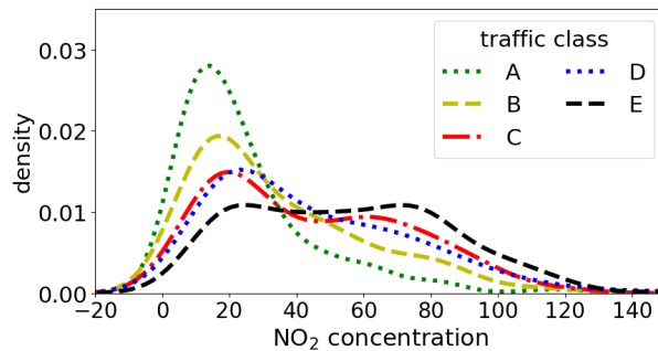
Figure 2. Training dataset, i.e., pollution data distribution given road traffic class.
