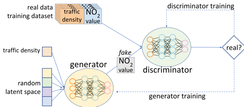
Figure 1. General CGANs training setups.
