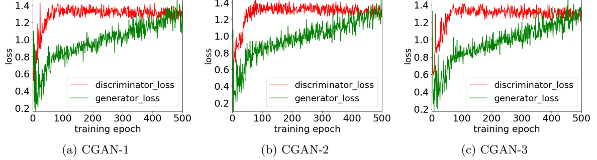
Figure 3. Discriminator and generator loss values through the training process.
