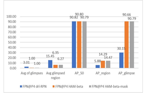
Figure 2: Comparisons between different configurations for the proposed model and peer methods.
