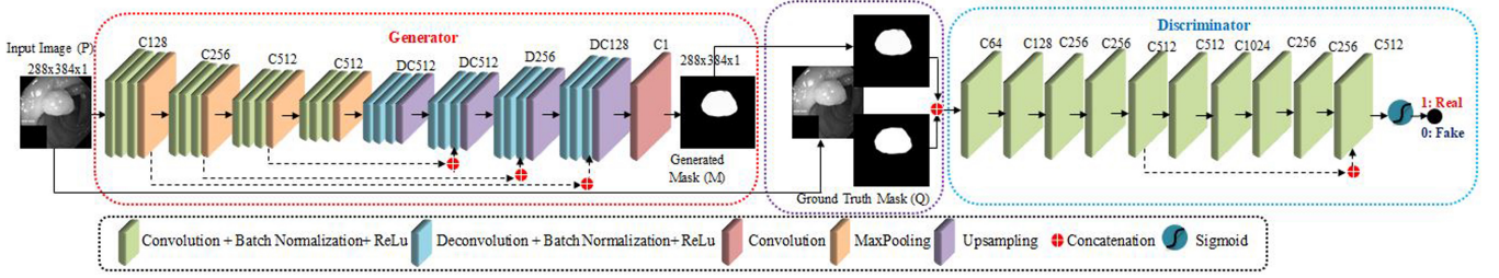
Figure 1: Proposed Framework for segmentation of polyp
