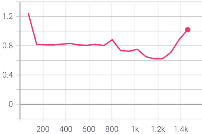
Figure 2: Validation Loss
