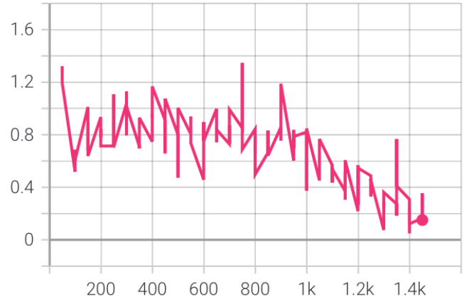
Figure 1: Training Loss
