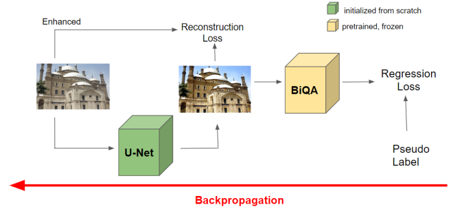
Figure 1: Vanilla End-to-End method
