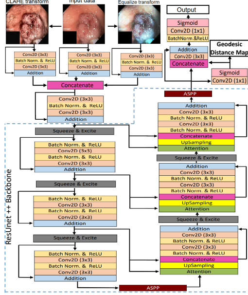
Figure 1: ResNet++ with Triple-Path and Geodesic distance
