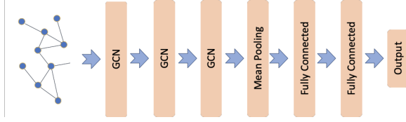
Figure 1: GCN architecture from [3]
