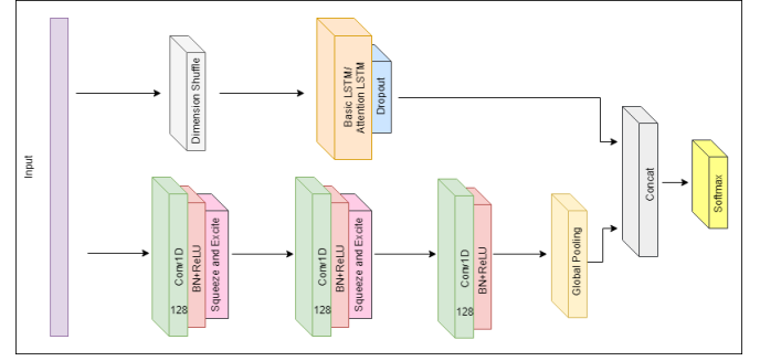
Figure 3: MALSTM-FCN architecture from [6]
