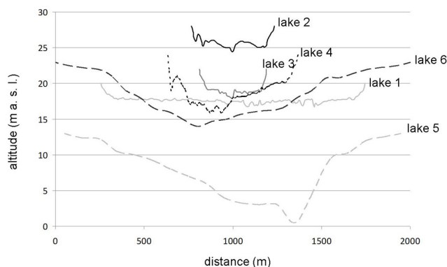
Fig. 8. Bathymetric profiles of lakes in relation to relief position. For lake locations see Fig. 4. Lake areas and profile directions are as follows: lake 1 = 1841 400 m 2 , from N to SE; lake 2 = 104 400 m 2 , from N to S; lake 3 = 221 400 m 2 , from N to S; lake 4 = 421 200 m 2 , from N to S; lake 5 = 1 636 790 m 2 , from NW to SE; lake 6 = 2 460 134 m 2 , from N to S. Bathymetric data from lakes 5 and 6 from Pavlova and Dorozhkina (2000).
