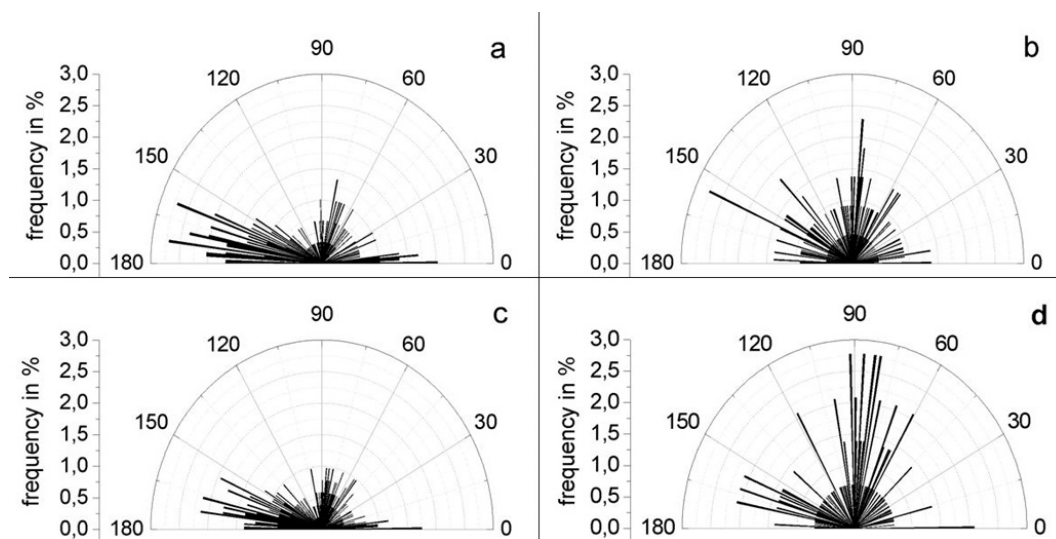
Fig. 6. Frequency distribution of major axis orientation for (a) lakes \geq 14\,400\text{ m}^2 on Yedoma uplands, (b) lakes \geq 14\,400\text{ m}^2 in basins, (c) all lakes \geq 14\,400\text{ m}^2 , and (d) single basins. Intervals = 1^\circ , 0^\circ = East, 90^\circ = North, 180^\circ = West.
