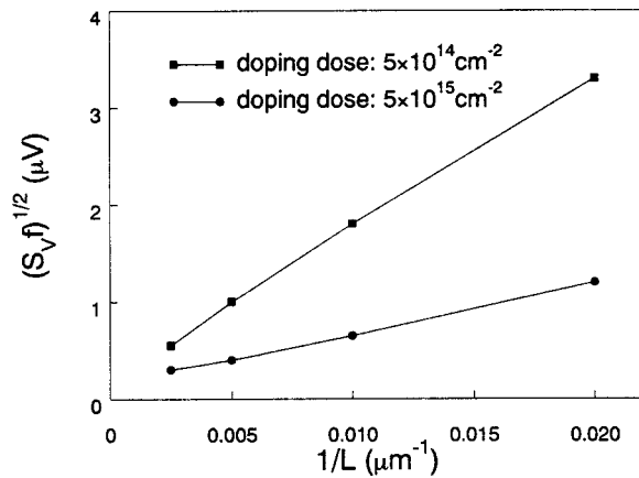
FIG. 5. Noise level comparison of two groups of amorphous silicon samples at two doping doses. The piezoresistor dimension is L/W = 10 , and annealed at 1050^\circ\text{C} for 30 min.
