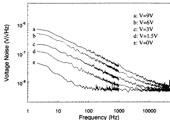
FIG. 7. Noise measurement spectra of an amorphous silicon sample at different biased voltages. The piezoresistor dimension is L/W = 5 , L = 100 \mu\text{m} , the doping dose is 5 \times 10^{15} \text{ cm}^{-2} , and annealed at 950^\circ\text{C} for 10 min.
