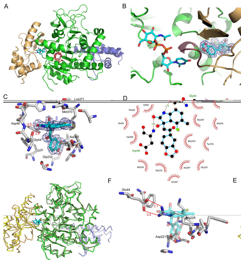
Figure 3. Structure of TbUAP in complex with 1 . (A) Overview of the TbUAP -1 structure (PDB ID 4bqh), which is composed of an N-terminal domain (beige), a central domain (green) containing the active site (nucleotide binding motif, red), and a C-terminal domain (blue). 1 (light blue) binds at an allosteric site. (B) 1 forms close contacts with a loop (PGGNG, dark red) between the N-terminal and central domain on the opposite face to the UDPGlcNAc binding site. The 2F_0 - F_c density of 1 is contoured at 1\sigma (dark blue mesh). Alignment of the TbUAP central domain with the CaUAP structure 2YQS 12 was used to model the UDPGlcNAc position. (C) Binding interactions of 1 with TbUAP , with the 2F_0 - F_c density of 1 displayed. (D) Schematic of the key interactions in the TbUAP -1 complex. (E) C- \alpha trace showing that the allosteric binding site of HsUAP is wider and flatter due to movement of the N-terminal domain. (F) Binding interactions in the modeled HsUAP -1 complex showing steric clashes produced by nonconservative substitution. Alignment of the TbUAP central domain with the HsUAP structure 1JV1 11 (gray) was used to model the binding of 1 (blue, transparent).
