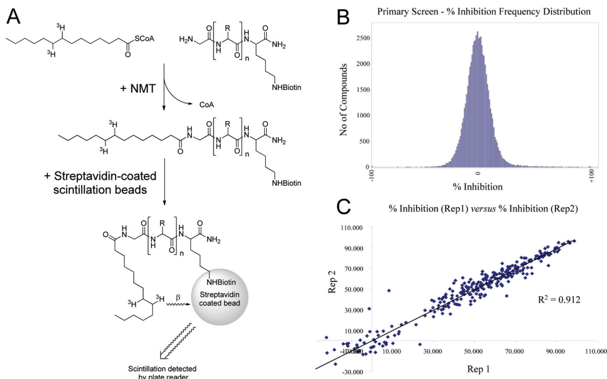
Figure 1. Format and performance of the HTS assay: (A) % inhibition and \text{IC}_{50} values determined using a scintillation proximity assay; 2 (B) frequency histogram representing % inhibition values for the HTS. Hits are designated as those compounds that displayed a % inhibition equal to or greater than 3 standard deviation units above the mean (40% inhibition). (C) Comparison of replicate % inhibition values for the 352 primary screen hits.
