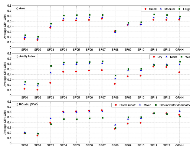
Fig. 4. Average of CR1–CR4 in validation in three classes of: (a) catchment area, (b) aridity index, and (c) RC_{S/W} .
