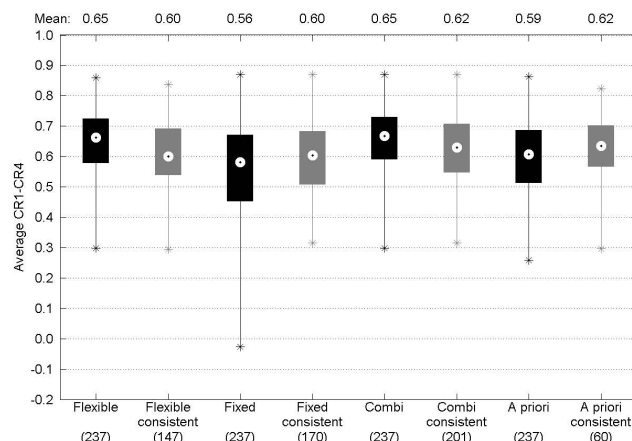
Fig. 6. Distribution of average performance in validation for the flexible, fixed, combined and a priori approaches. The whiskers denote the minimum and maximum values, the shaded boxes indicate the 25th–75th percentiles, and the circles indicate the median value. The dark boxes represent the distributions including inconsistent results, and the grey boxes represent only consistent results. The number of catchments in each group is given in brackets.
