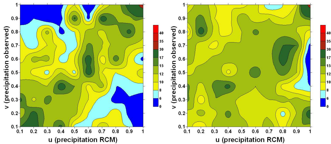
Fig. 8. Empirical Copula density for modelled ( u ) and observed precipitation ( v ) for station Garmisch-Partenkirchen, using the positive pairs of original data (left), and the positive pairs of the ARMA-GARCH transformed iid residuals (right).
