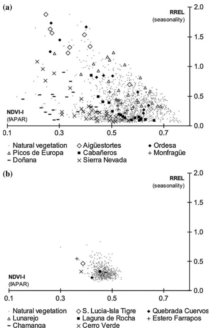
Fig. 2 Analysis of representativeness of Spanish national parks (a) and Uruguayan candidate protected areas (b) based on ecosystem functional attributes derived from remote sensing. For each country, the approach locates the protected areas in the functional space defined by the whole range of annual NDVI integrals (NDVI-I, an estimator of annual C gains) and the relative range of variation in light interception during the year (RREL, an indicator of seasonality). Points correspond to the discrete area defined by a pixel. Grey points correspond to natural (non-agricultural) areas. Protected sites coincident with repetitive combinations of productivity and seasonality were considered representative, while sites corresponding to unique or rare combinations were considered singular. (Adapted from Cabello et al. 2008)
