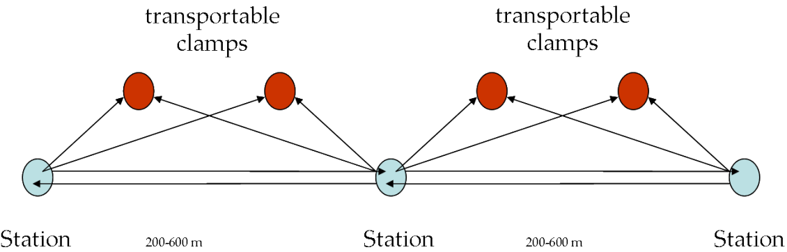
Figure 2: The traverse surveying pattern
