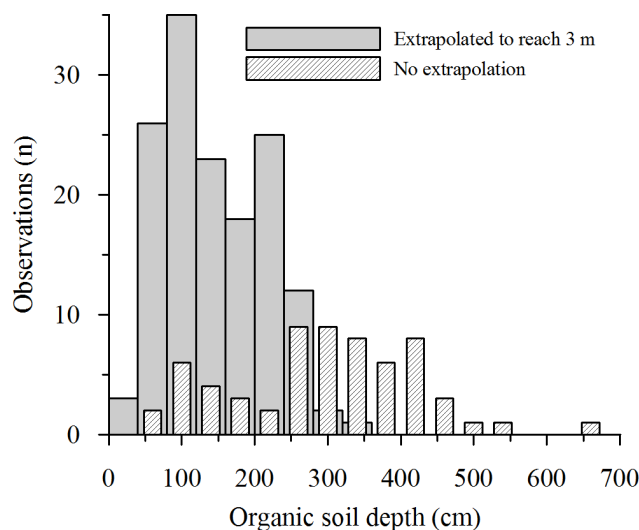
Figure 4. Histograms illustrating the depth-distribution of peat deposits (organic soil material) in Histosols and Histels of pedon data set 2 (bins = 40 cm depth). The graph shows separate histograms for pedons that were extrapolated to reach the full 3 m depth required for upscaling and pedons where no extrapolation was needed.
