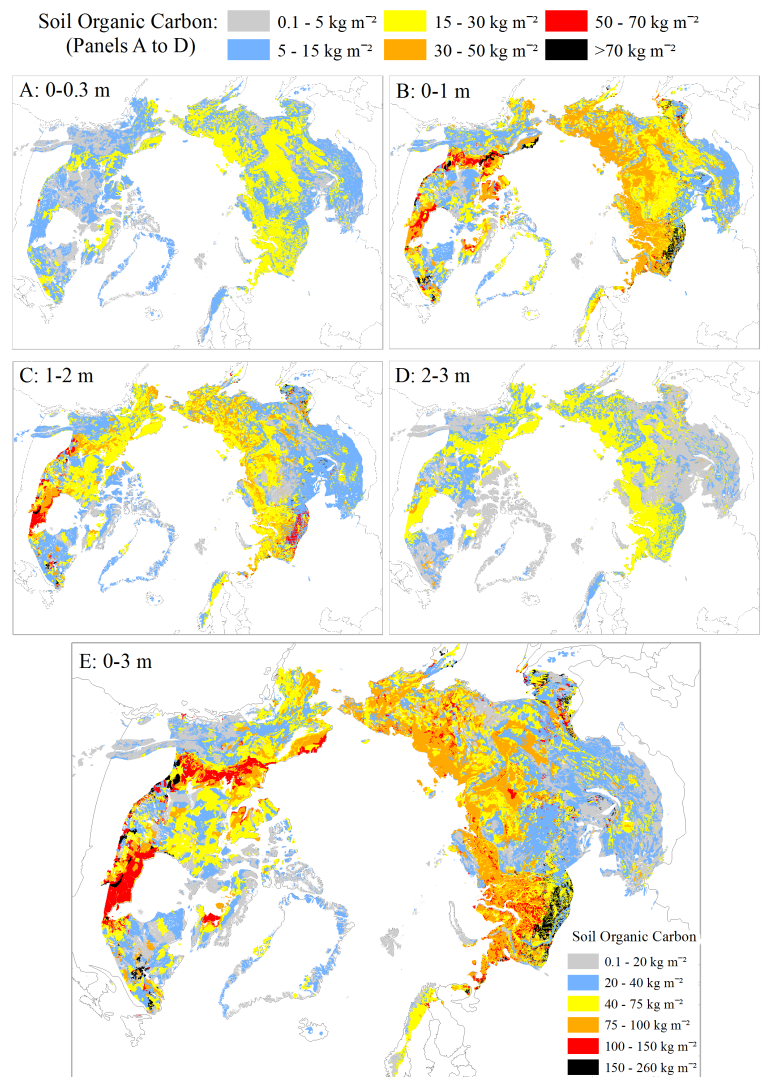
Figure 3. Map of estimated 0–3 m SOC storage ( \text{kg C m}^{-2} ) in the northern circumpolar permafrost region. Panels show 0–0.3 m and 0–1 m SOC calculated subdivided following NCSCD regions while 1–2 m and 2–3 m SOC is calculated subdivided for areas of thick thin sedimentary overburden. Projection: Azimuthal Equidistant, datum: WGS84.
