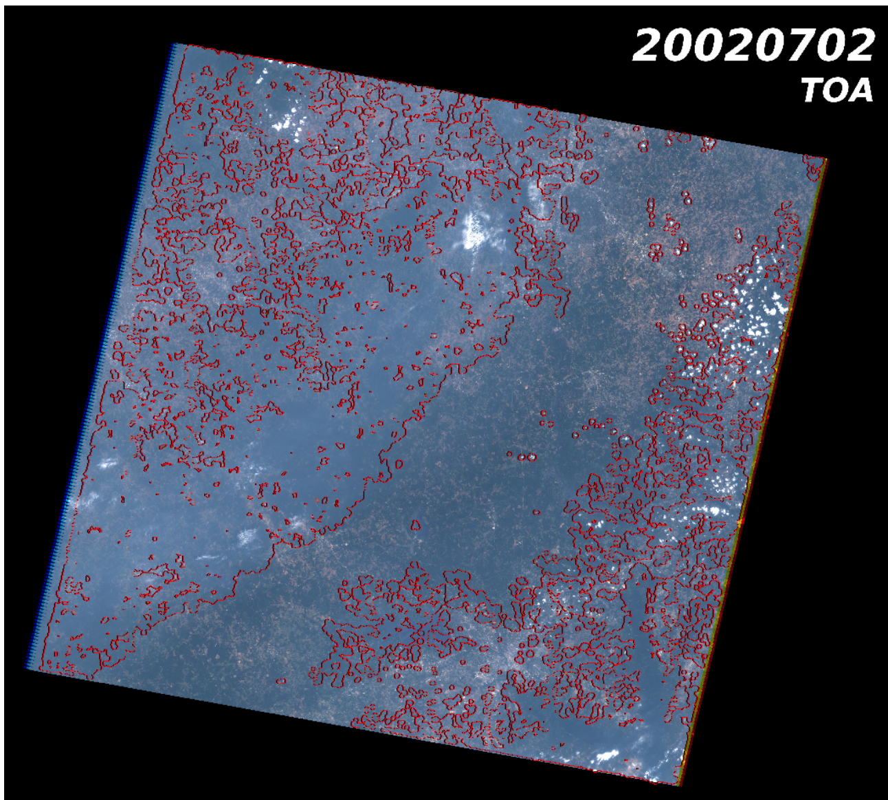
Figure 9 :LANDSAT 7 image near Columbia, South Carolina, USA, for which cloud cover is 1.7% according to data catalogue and 51% according to MTCD method. Red lines correspond to MTCD image contours. Although the result of MTCD method is maybe too strict, and its appreciation might be subjective, the ACCA percentage is clearly underestimated.
