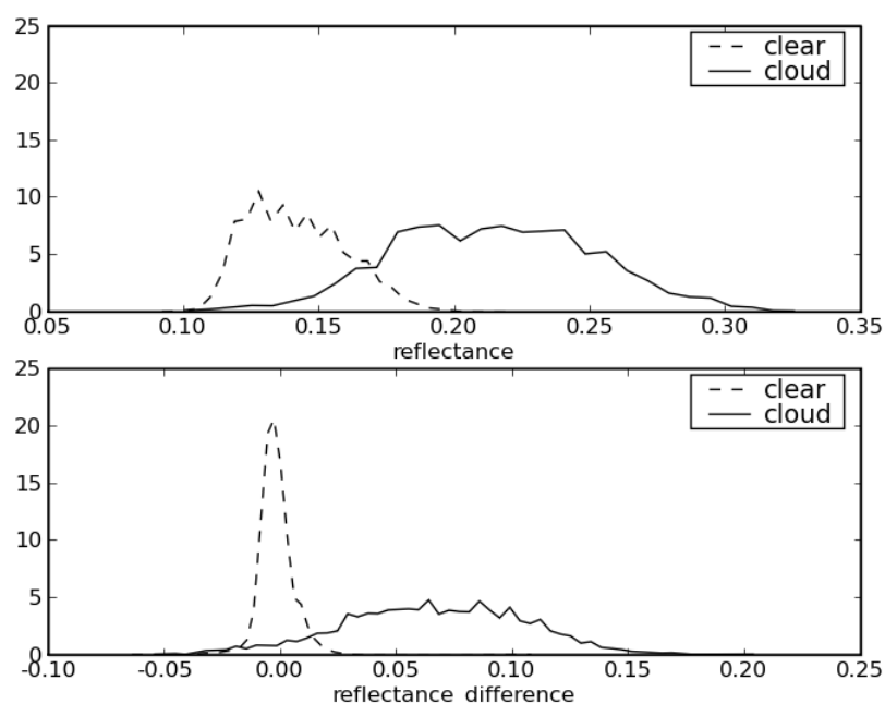
Figure 1 :Comparison of histograms of clouded and unclouded pixels for FORMOSAT-2 blue band on Tensift site (Morocco), top : absolute reflectance on the April 13th, 2006, bottom: reflectance variation between the April 1 st and the April 13th 2006. The image on April 1 st is completely cloud free. Pixels within cloud shadows are not taken into account in the histograms.
