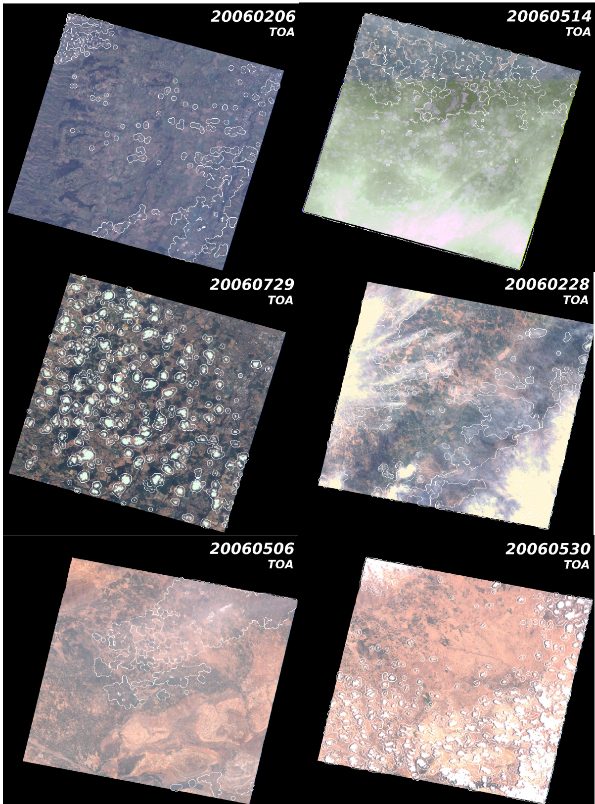
Figure 5 : visual verifications for a few cases identified in figure 3. White lines correspond to cloud contours from MTCD method. Upper Left) MTCD gives 12% of cloud cover, NSPO: 0%. Very small clouds can be seen, that were not seen by the operator. Upper Right) MTCD 80%, NSPO: 20%. Here, the operator probably only considered the thick clouds at the bottom of the image, but most of the image is evidently covered by thin clouds. Middle left) MTCD : 34%, NSPO 55%. The image is covered by small clouds, all of them seem to have been detected by MTCD. The operator has probably considered part of the space between clouds as cloudy. Middle right) MTCD 37%, NSPO 85%, the thin cloud cover is underestimated by our cloud mask because the previous image in the time series is quite old. Bottom Left) MTCD 22%, NSPO 0%. Thin clouds were not classified as clouds by NSPO operator. Bottom Right) MTCD 42%, NSPO 20%. The MTCD cloud cover looks accurate.
