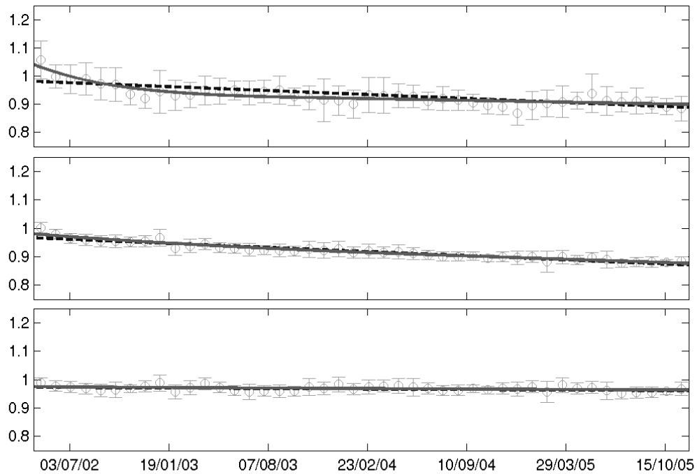
Figure 1. Time course of the calibration coefficient obtained using 20 desert sites (Cabot et al., 2000; Hagolle et al., 1999) for VEGETATION 2 using POLDER 2 as a reference: top: Blue band (B0); centre: red band (B2); bottom: near-infrared band (B3). The calibration coefficient corresponds here to the correction to apply to the pre-launch calibration of VEGETATION2. Symbols are monthly averages with standard deviation, and curves are the best fit of a linear model (dashed line) or the non linear model (plain line).
