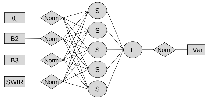
Figure 6. Architecture of the neural network used to estimate LAI , fAPAR and fCover (here labelled Var) from VEGETATION normalized top of canopy reflectance in bands B2, B3 and SWIR. Sun zenith angle ( \theta_s ) corresponding to the median value during the compositing period is also used as input. ‘Norm’ corresponds to the normalization of the inputs and outputs. Neurones with ‘S’ and ‘L’ mean respectively tangent-sigmoid and linear transfer functions.
