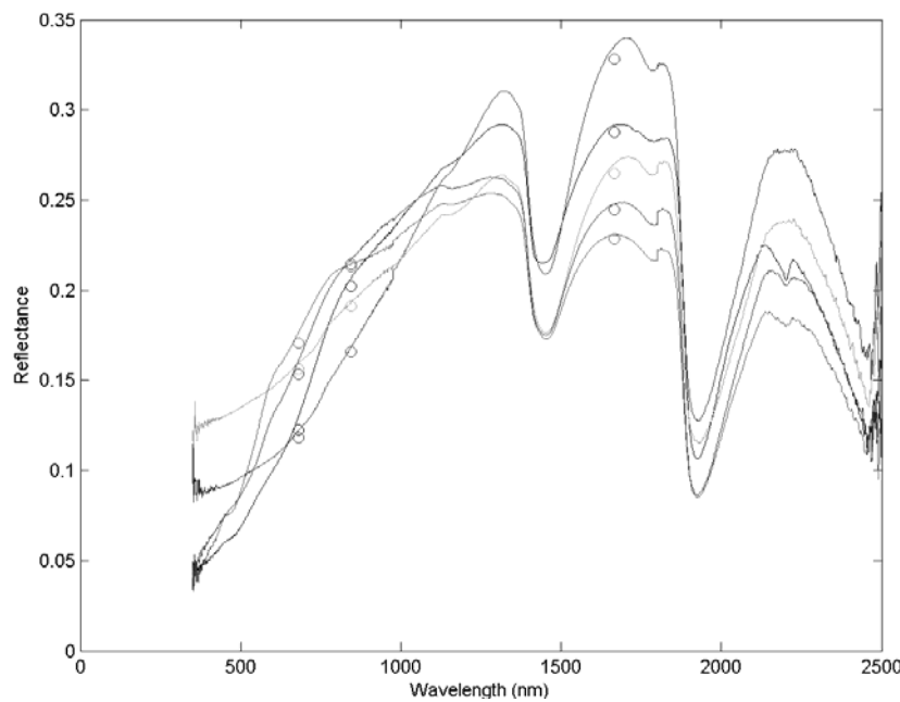
Figure 3. Reflectance of the 5 soils used to represent the possible range of spectral shapes.
