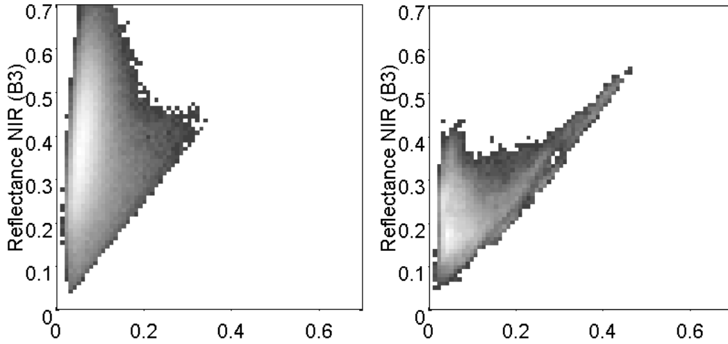
Figure 4. On the left, density plots of simulated reflectance values in red (B2) and near infrared (B3) feature plan (196608 cases). On the right, the same figure with actual VEGETATION data acquired over a subset of 196608 pixels randomly selected over the BELMANIP sites for years 1999-2003 and for which water bodies, cloud and snow contaminated pixels were eliminated as far as possible.
