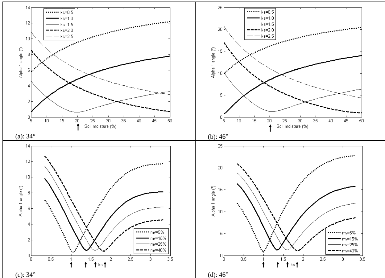
Fig. 4. Behaviour of \alpha_1 from the RADARSAT-2 data as a function of the soil moisture and ks .
