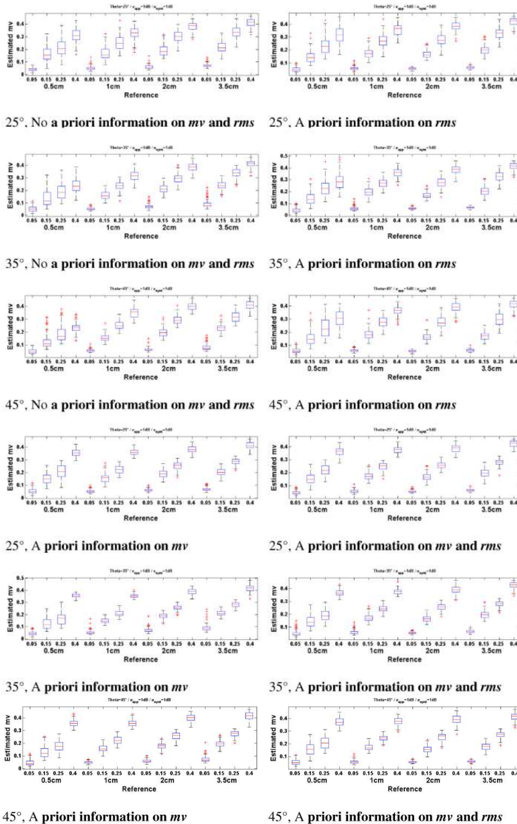
Fig. 2. Box plots of soil moisture estimates (cm 3 cm -3 ) retrieved from the synthetic dataset. Training and validation datasets correspond to a noise on the backscattering coefficients of \pm 1 dB. Four rms and four mv values were plotted: rms = 0.5, 1, 2, 3.5 cm; mv = 0.05, 0.15, 0.25, 0.40 cm 3 cm -3 .
