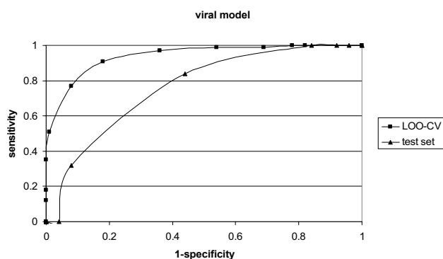
Figure 2 ROC curves for Vaxijen viral model.
