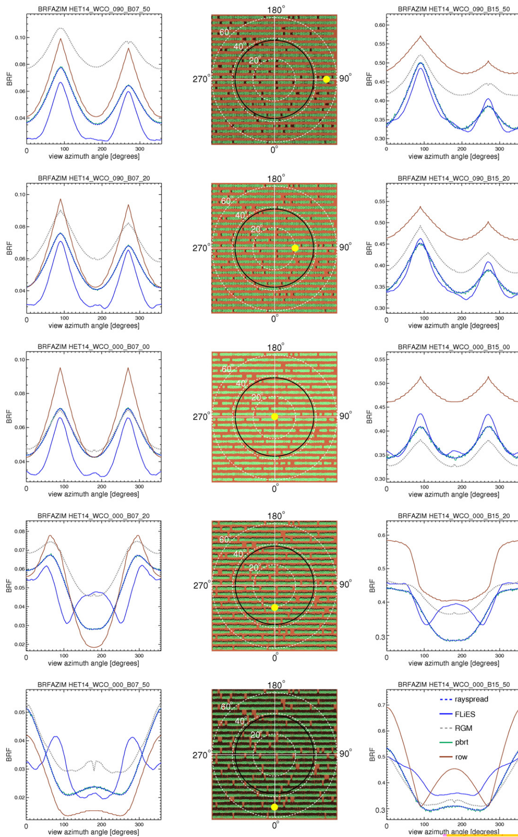
Fig. 4. Model simulations in band 7 (661 nm; left column) and band 15 (865 nm; right column) of the BRF leaving the Wellington Citrus Orchard scene at a constant view zenith angle of 37° and view azimuth angles from 0 to 360°. Graphical depictions of the target canopy when viewed from nadir are shown in the middle column, together with a (white coloured) polar coordinate system indicating the viewing (black ring) and illumination (yellow disc) configuration with respect to the planting pattern.
