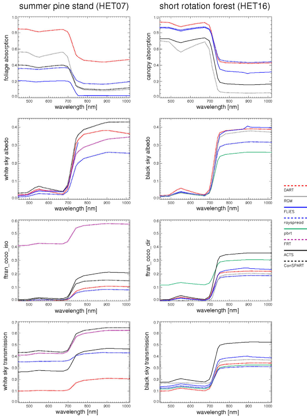
Fig. 5. Examples of model simulated flux spectra pertaining to the HET07 Järvselja pine stand (left column) and the HET16 Lombardy short rotation forest illuminated with a zenith angle of 50° perpendicular to the row orientation (right column). The simulations cover the wavelength range from 442 nm (B1) to 1019 nm (B18). The first row depicts absorption quantities, the second albedo quantities and the last total transmission quantities. The third row depicts that transmission component which has undergone at least one scattering interaction on its way down through the canopy for isotropic diffuse incident radiation only (left panel) and direct incident radiation only (right panel).
